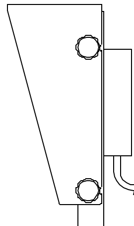
OPTIONAL SUN SHADE INSTALLED
